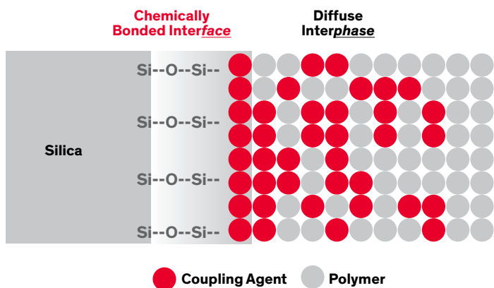
Figure 4: The inter-penetrating network (IPN) bonding mechanism
