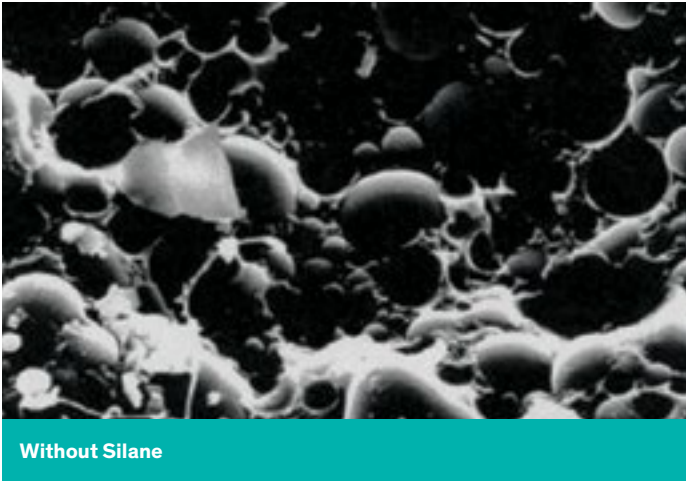
Figure 2: SEM image of silica-filled epoxy resin
